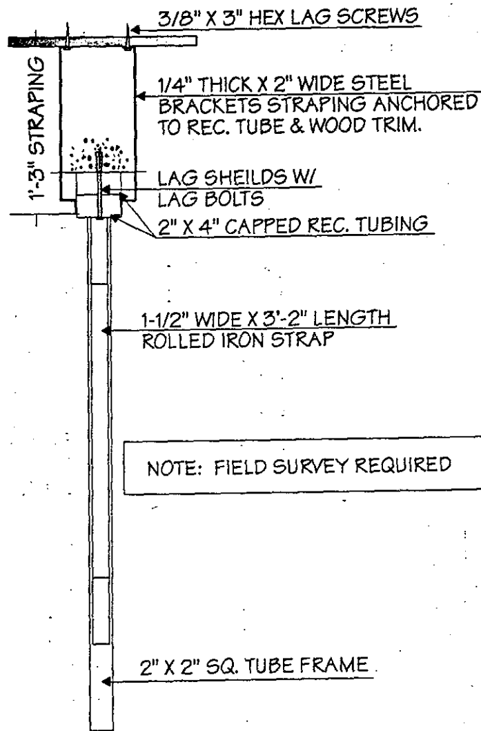
PLAN VIEW / INSTALL DETAIL SCALE 1" = 1'-0"
