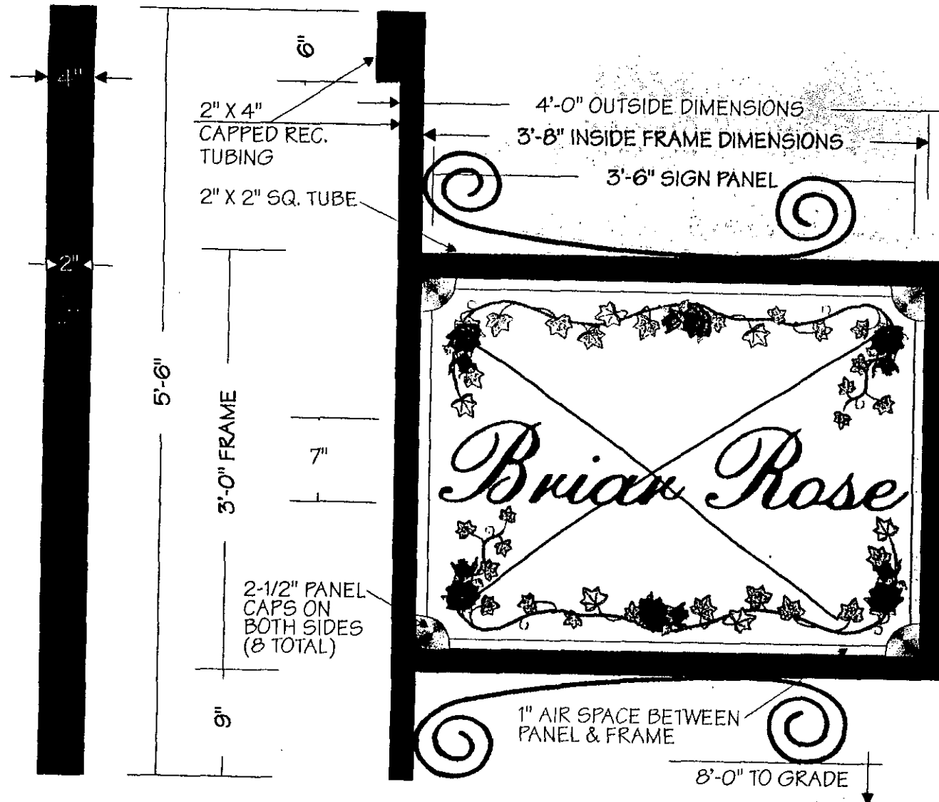
B NEW D/F NON-ILLUMINATED CANTILEVER MOUNTD ALUM. PANEL W/ SQ. TUBE FRAME SCALE 1" = 1'-0"
