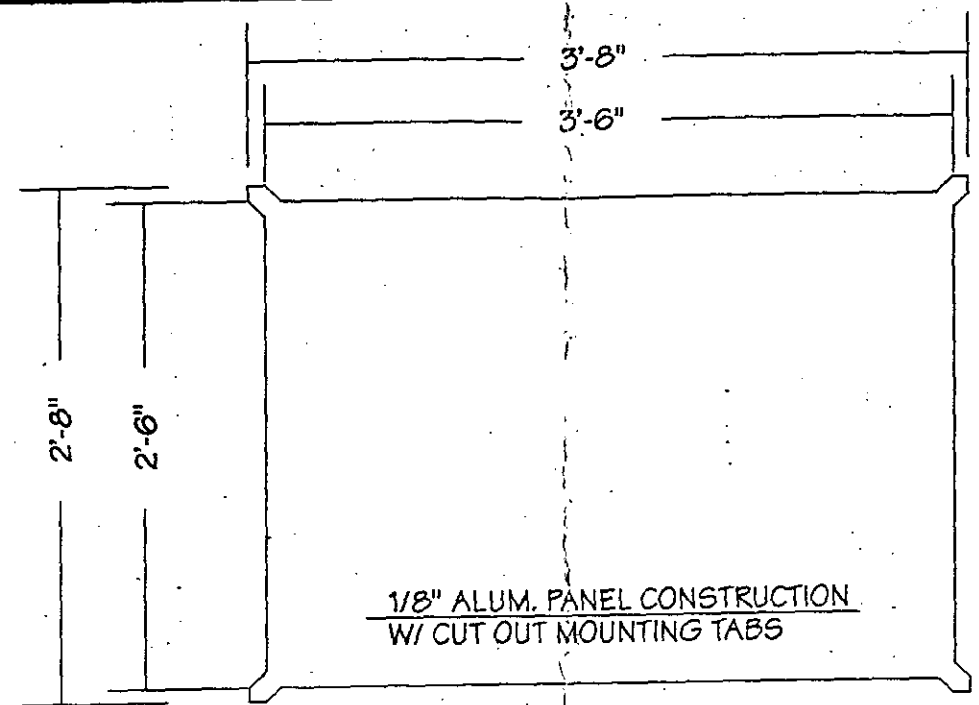
ALUMINUM GRAPHICS PANEL DETAIL SCALE 1" = 1'-0"
