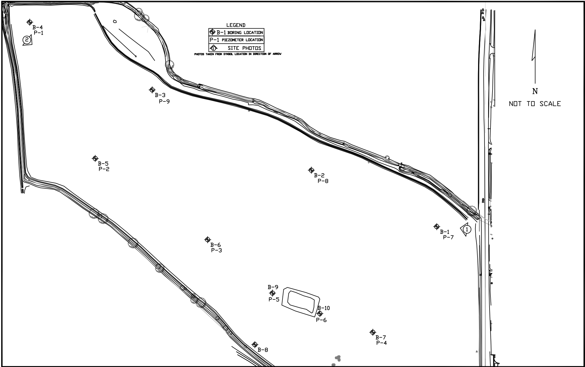
BORING LOCATION DIAGRAM HANSEN PROPERTY – LARIMER COUNTY, COLORADO EEC PROJECT # 1052066 SEPTEMBER 2005
