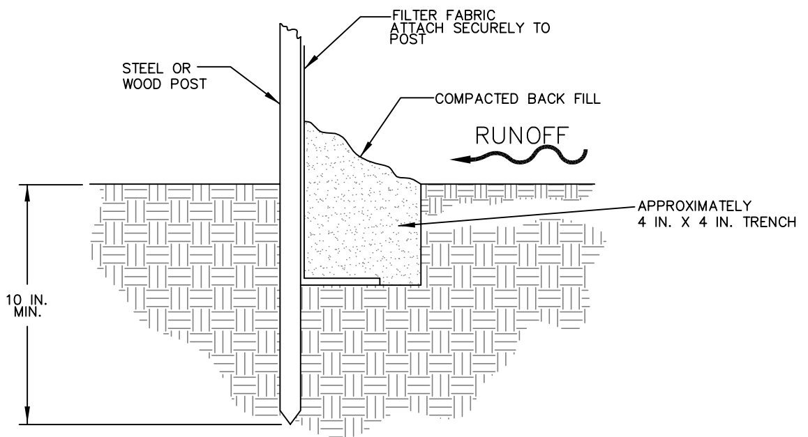
SECTION VIEW
