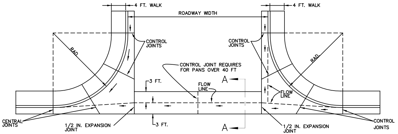
PLAN VIEW VERTICAL CURB, GUTTER AND SIDEWALK
