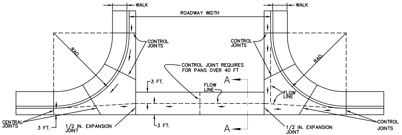
PLAN VIEW DRIVE-OVER CURB, GUTTER AND SIDEWALK
