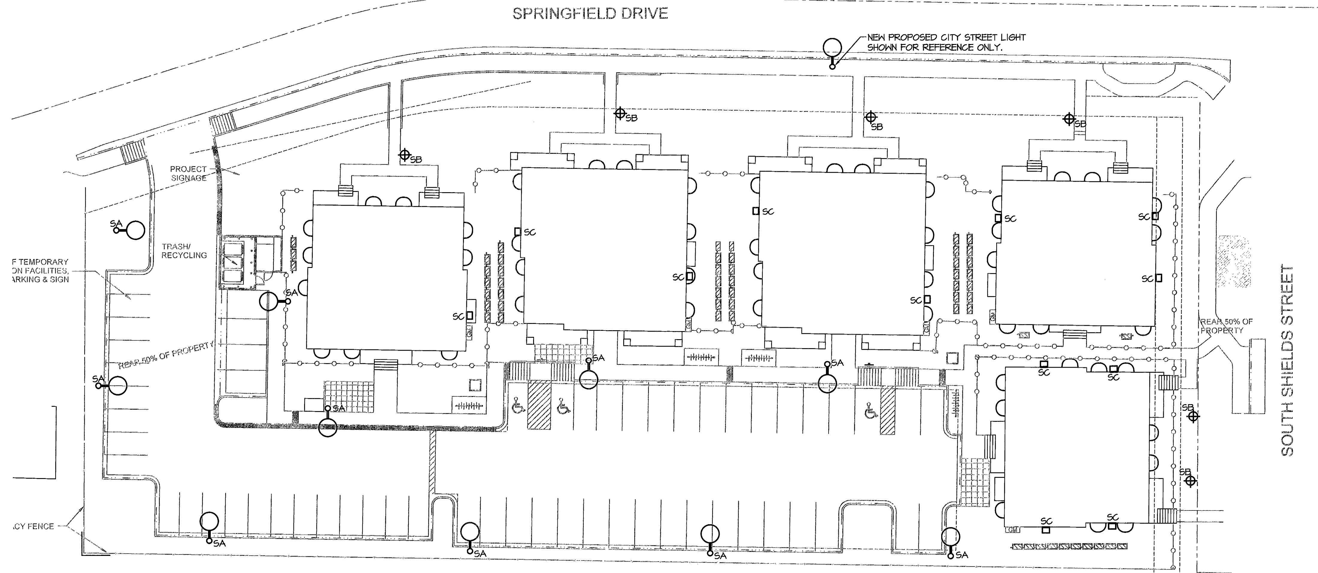
1 SITE LIGHTING PLAN 1"=20'-0"
