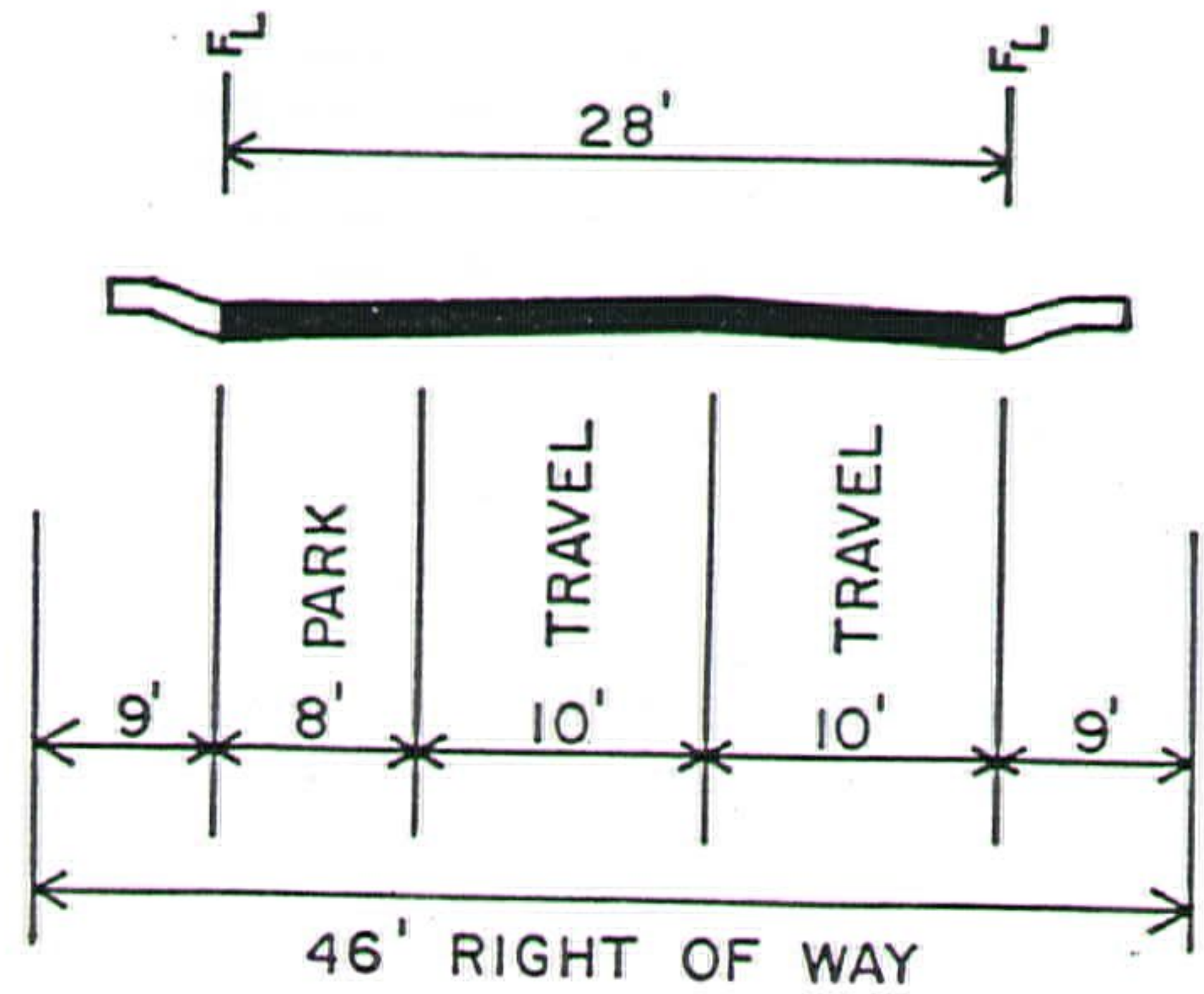
RESIDENTIAL (PUD'S ONLY)
