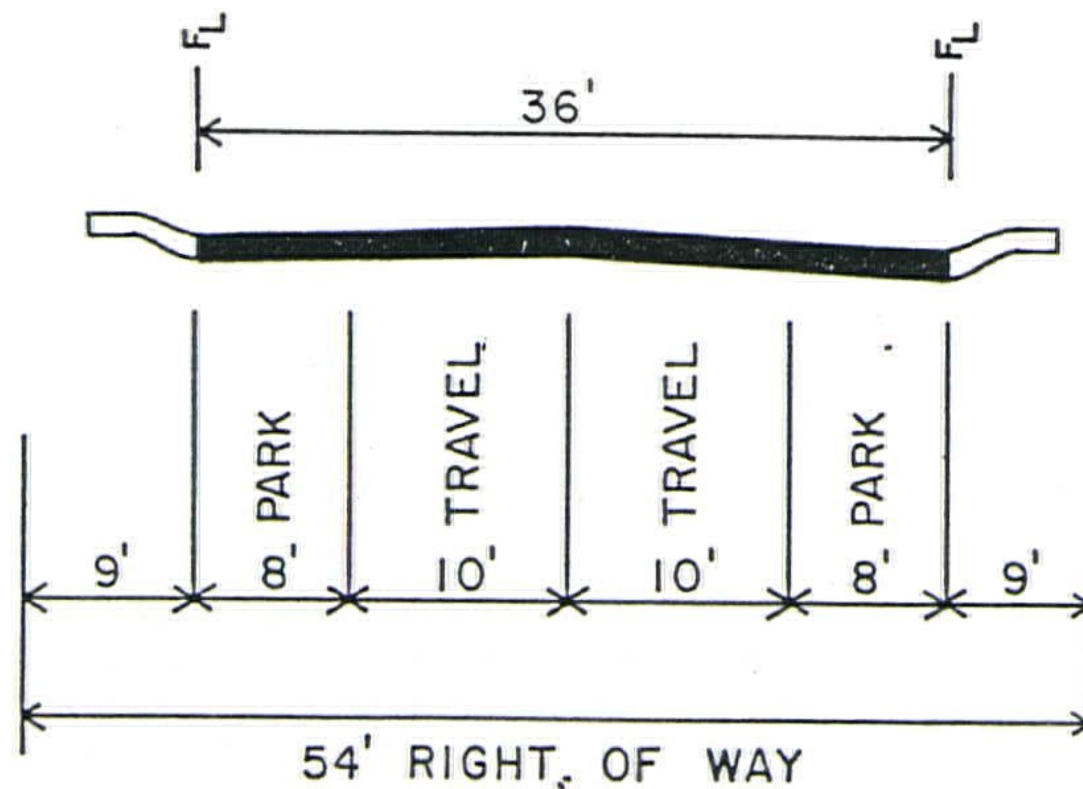
RESIDENTIAL (WITH PARKING)
