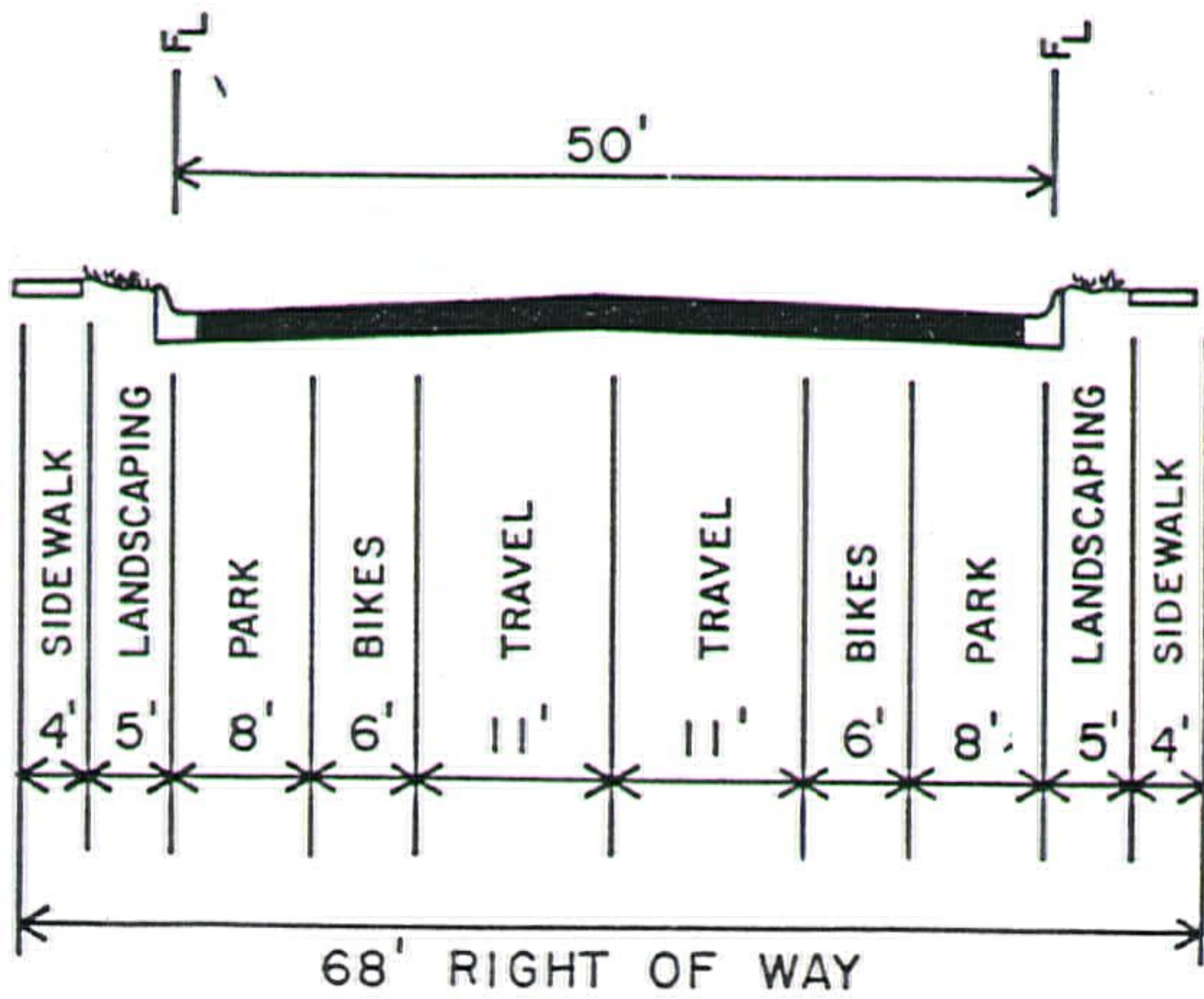
COLLECTOR (WITH PARKING AND BIKE LANES)
